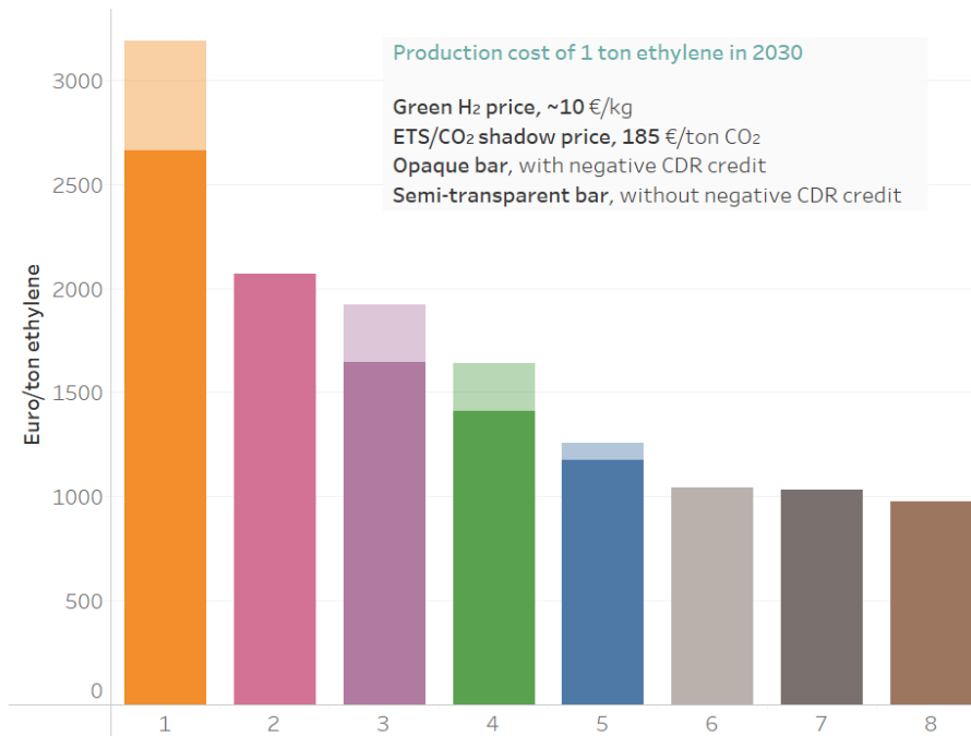
Figure 26. Ethylene production routes and cost in TCR by 2030. Own modelling work, based on [102].
